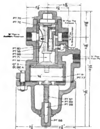
Fig. 2574. Plain Triple Valve, Type C, for 12-in., 14-in., and 16-in. Cylinders.
